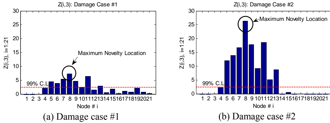
Figure 13: Novelty Index Z(i,3)
