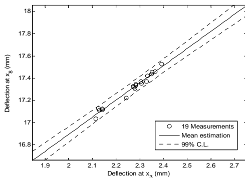
Figure 2: Typical example for the correlated deflection under the temperature variations
