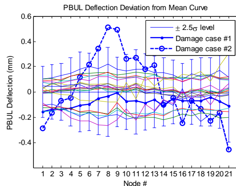
Figure 11: Deviation of Intact deflection
