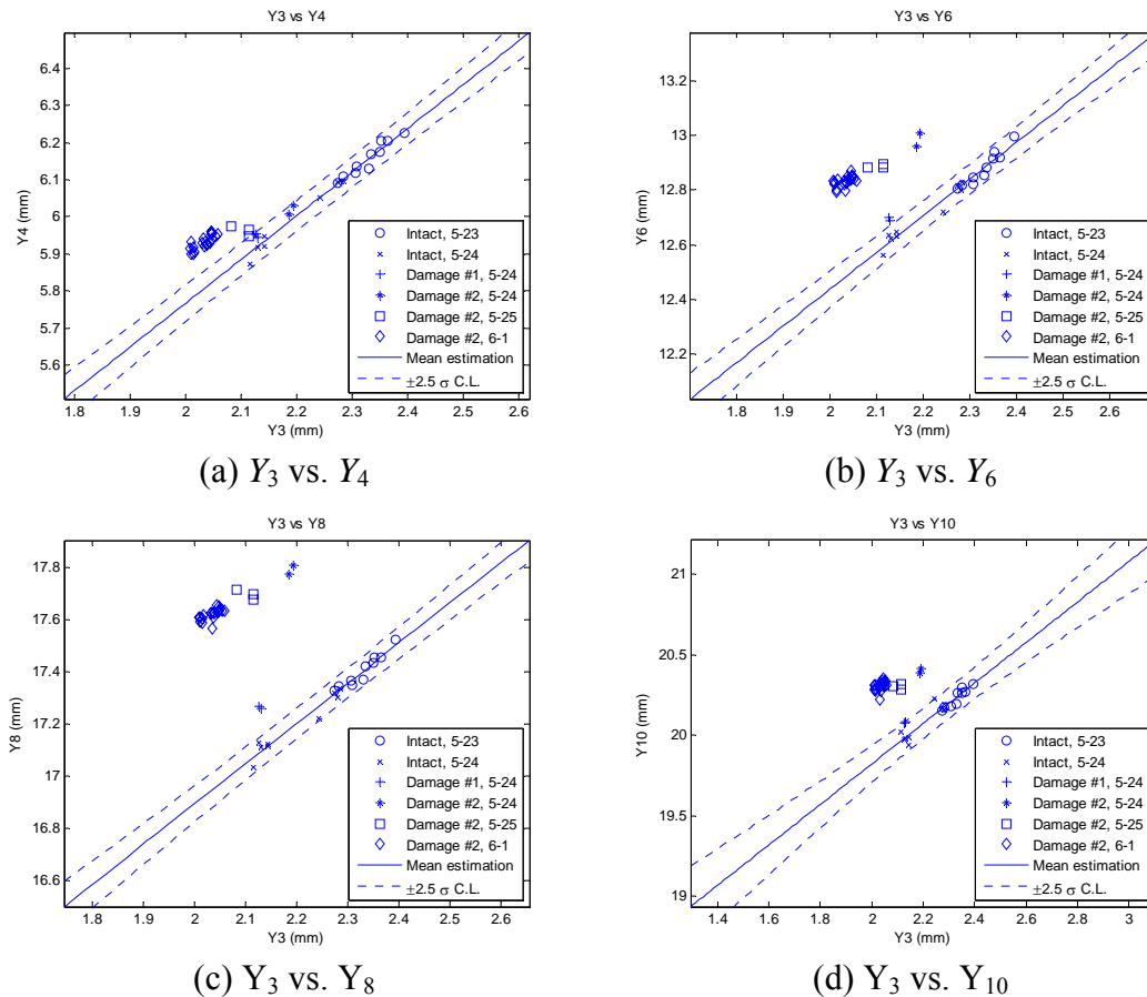
Figure 12: The outlier analysis for the correlated deflections
