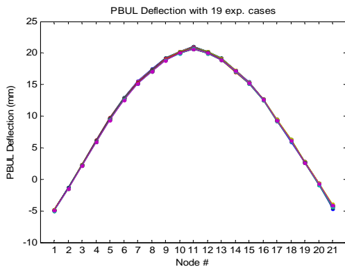
Figure 10: PBUL deflections (Intact case)
