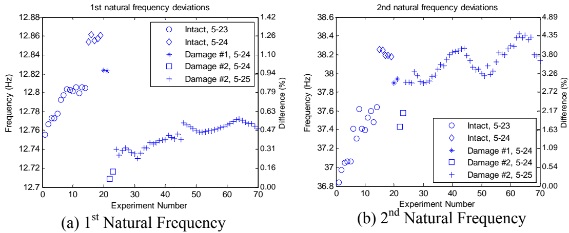
Figure 8: Deviation of natural frequencies under the temperature variation
